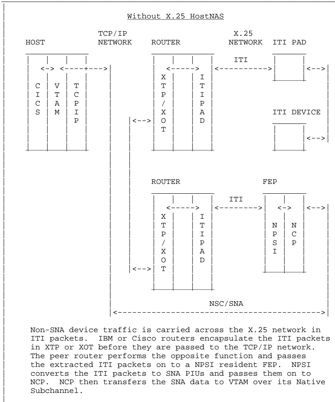
Figure 2: Non-SNA traffic in a hybrid X.25-TCP/IP Network without HNAS
